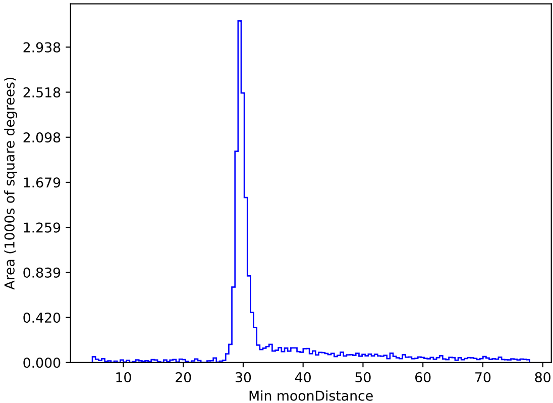
too_elab_r64_d2_griz_v3.4_10yrs WFD z band: Min moonDistance
