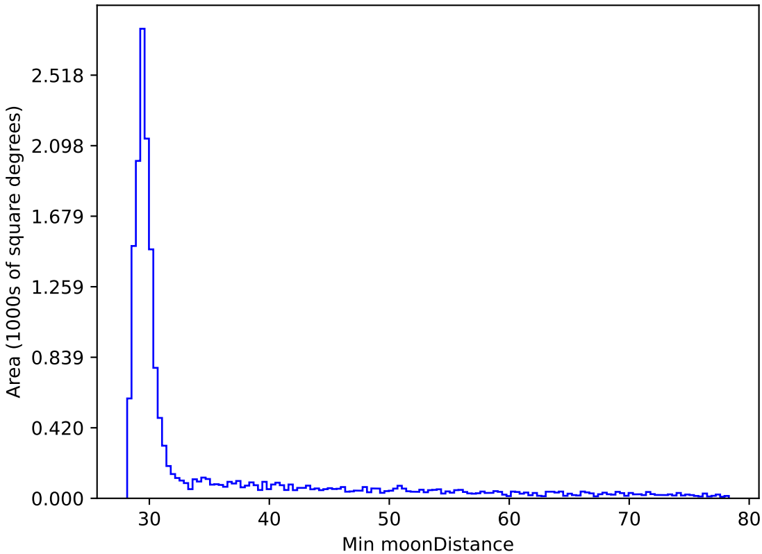
too_elab_r64_d2_griz_v3.4_10yrs WFD y band: Min moonDistance
