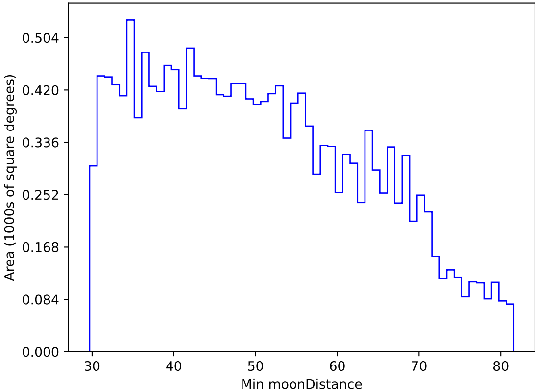
too_elab_r64_d2_griz_v3.4_10yrs WFD u band: Min moonDistance
