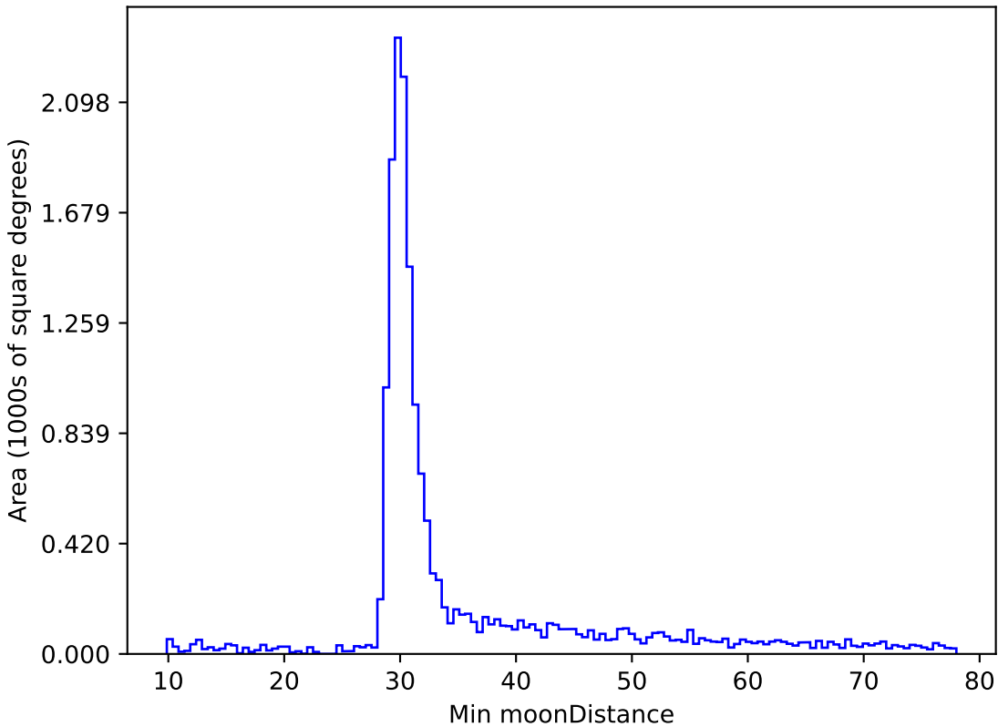
too_elab_r64_d2_griz_v3.4_10yrs WFD i band: Min moonDistance
