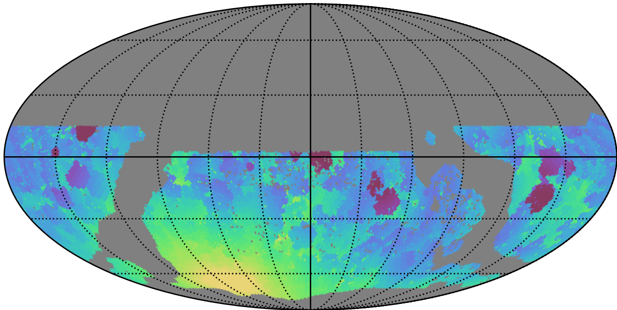
too_elab_r64_d2_griz_v3.4_10yrs WFD g band: Min moonDistance
