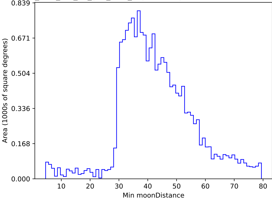
too_elab_r64_d2_griz_v3.4_10yrs WFD g band: Min moonDistance
