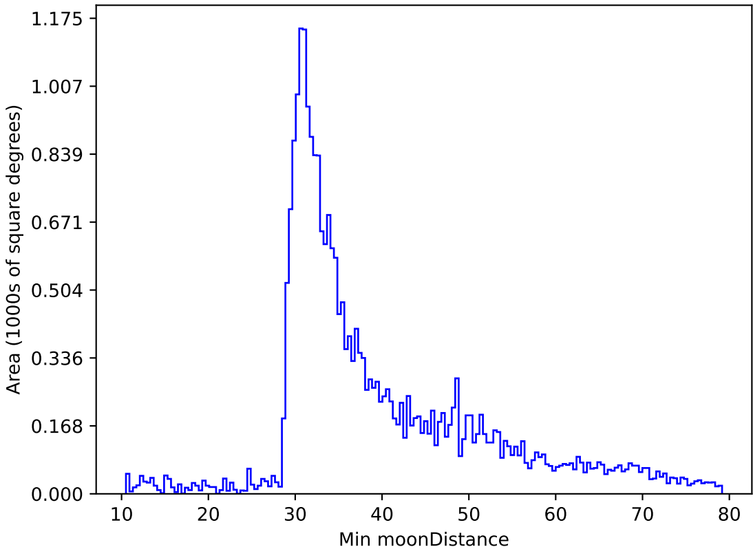
too_elab_r64_d2_griz_v3.4_10yrs All sky r band: Min moonDistance
