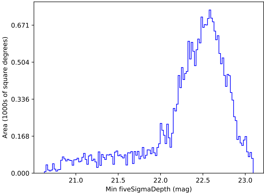
too_elab_r64_d2_griz_v3.4_10yrs Yr 1 z band: Min fiveSigmaDepth
