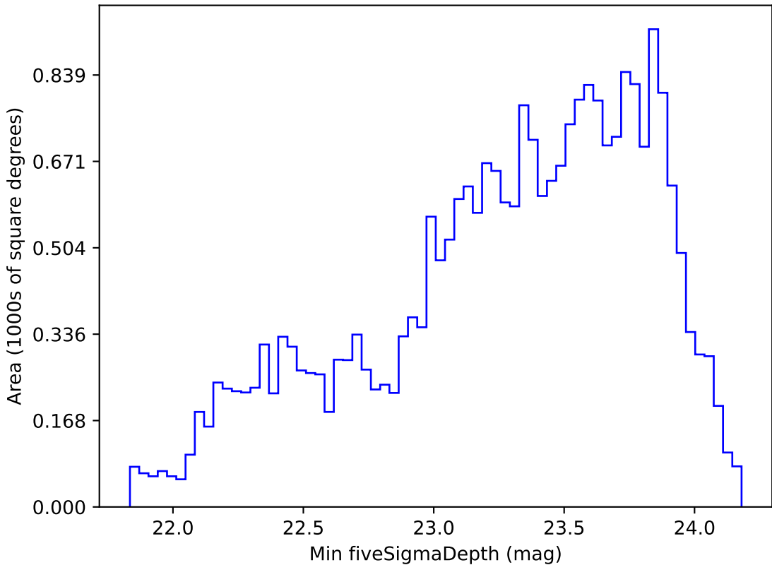
too_elab_r64_d2_griz_v3.4_10yrs Yr 1 r band: Min fiveSigmaDepth
