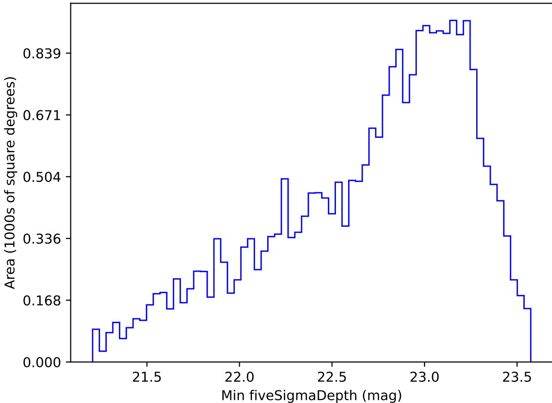
too_elab_r64_d2_griz_v3.4_10yrs Yr 1 i band: Min fiveSigmaDepth
