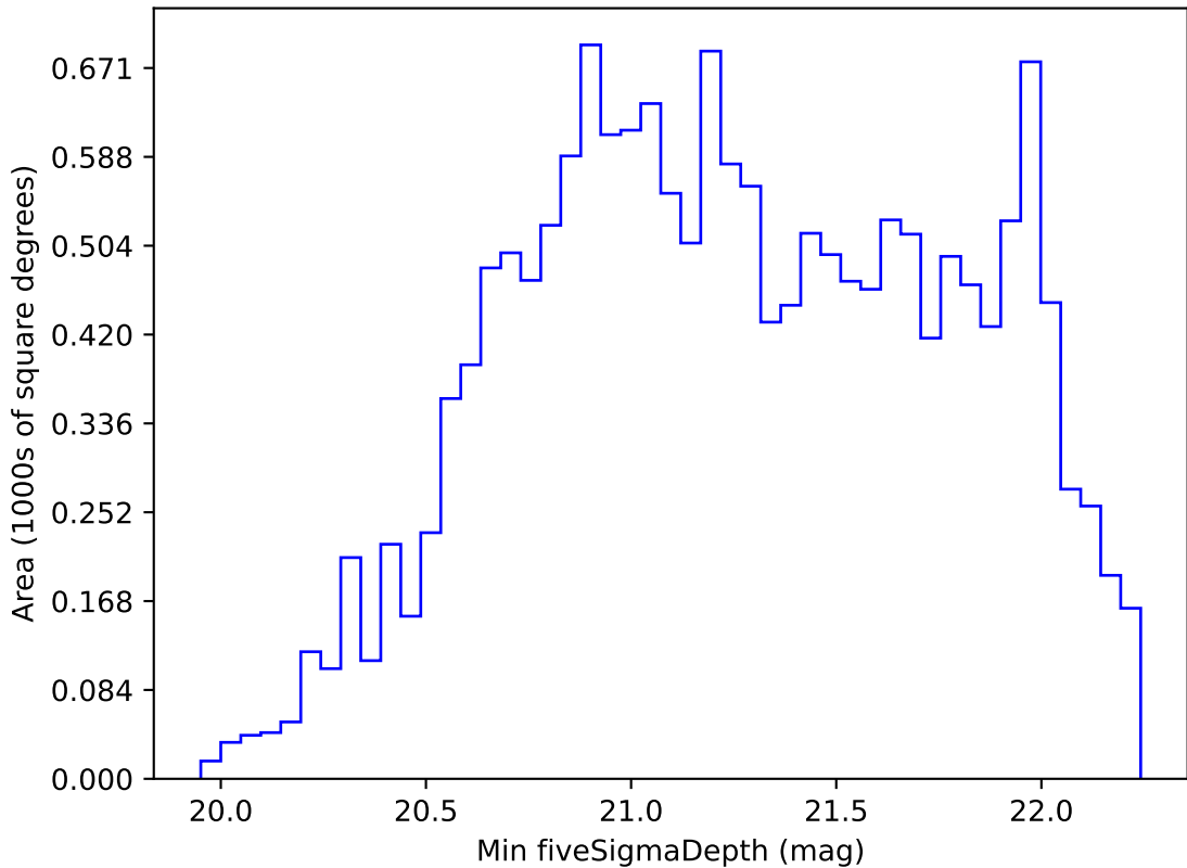
too_elab_r64_d2_griz_v3.4_10yrs WFD z band: Min fiveSigmaDepth
