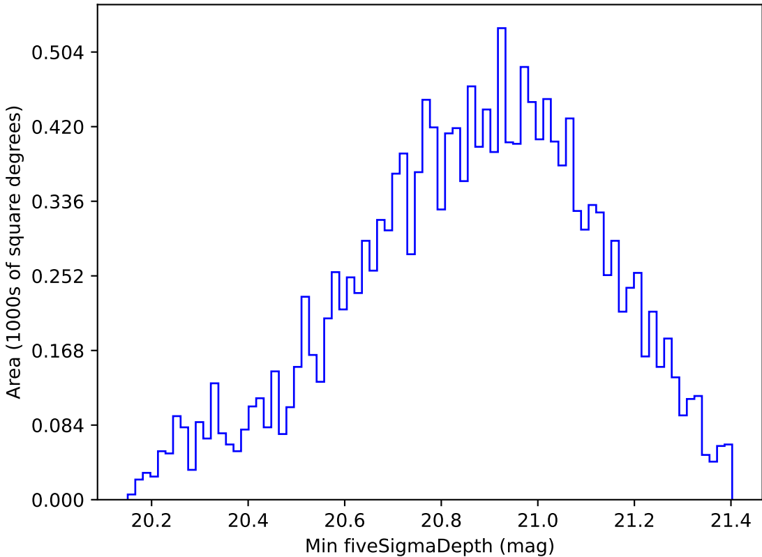
too_elab_r64_d2_griz_v3.4_10yrs WFD y band: Min fiveSigmaDepth
