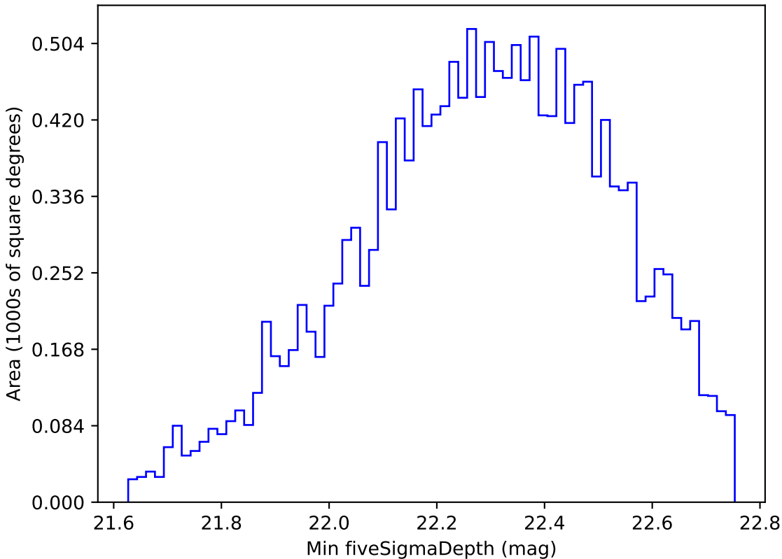
too_elab_r64_d2_griz_v3.4_10yrs WFD u band: Min fiveSigmaDepth
