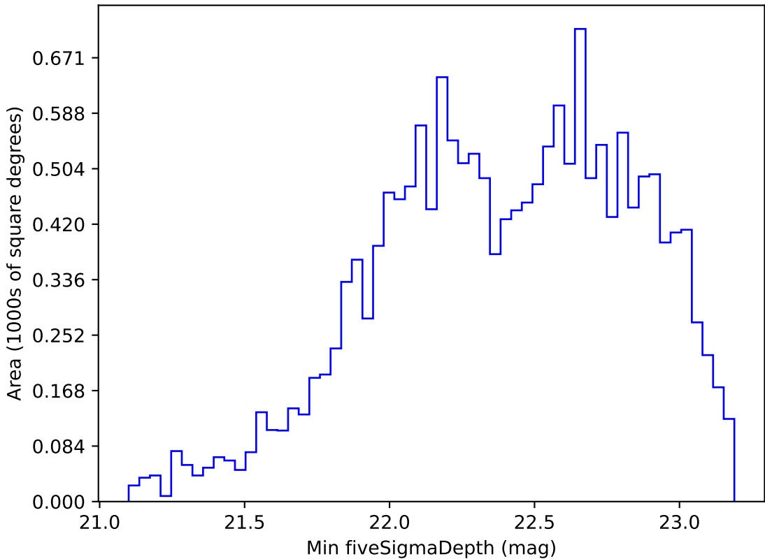
too_elab_r64_d2_griz_v3.4_10yrs WFD r band: Min fiveSigmaDepth
