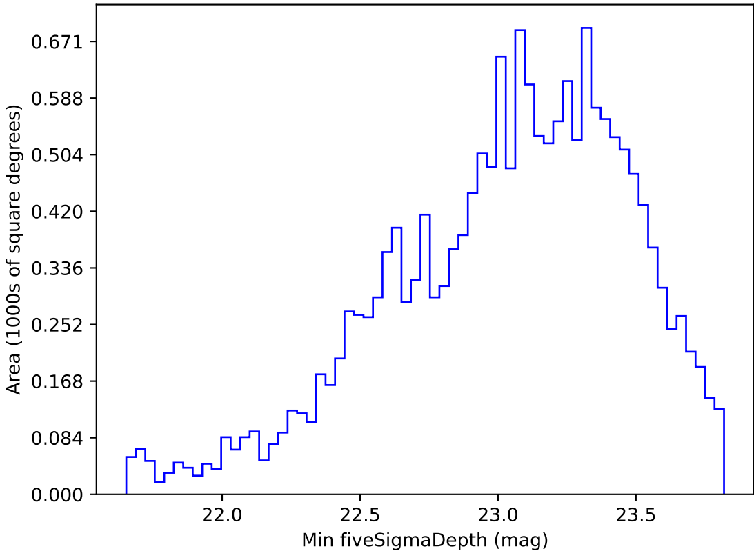
too_elab_r64_d2_griz_v3.4_10yrs WFD g band: Min fiveSigmaDepth
