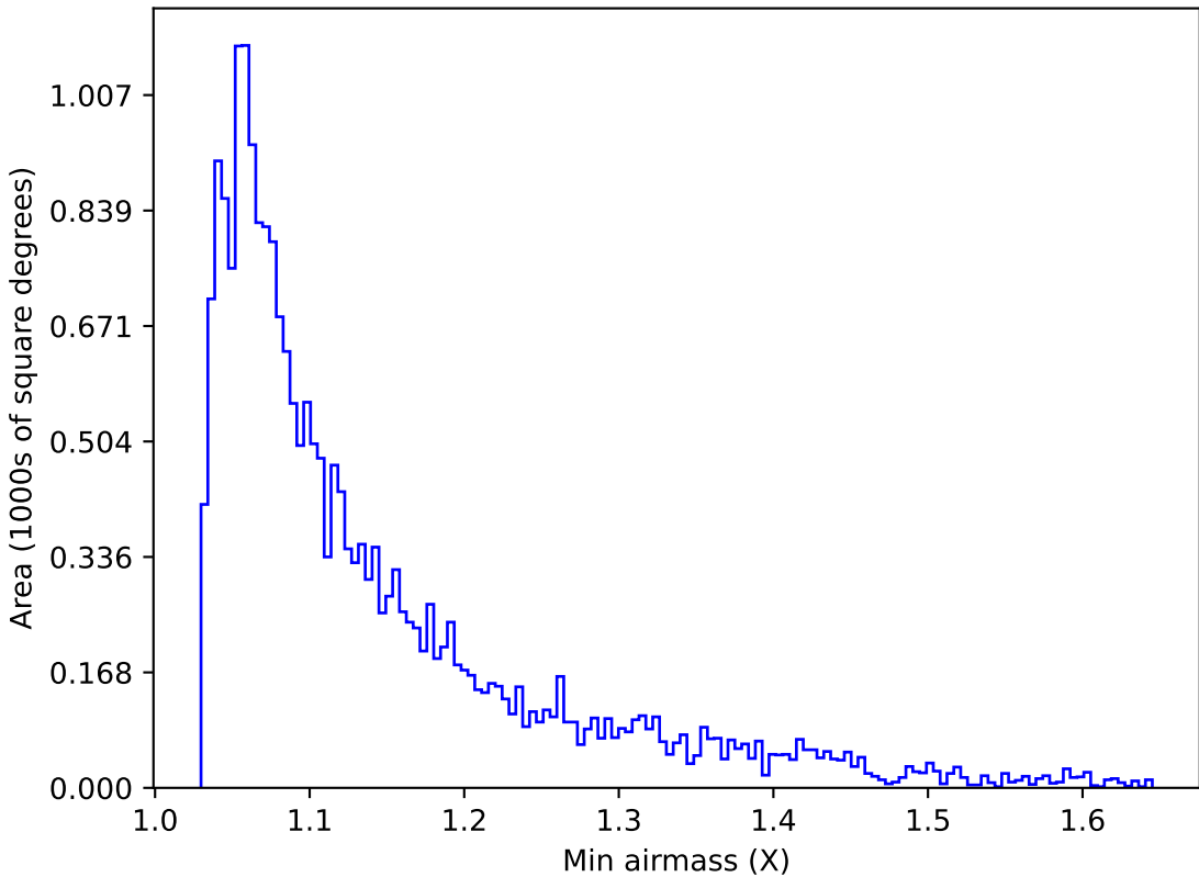
too_elab_r64_d2_griz_v3.4_10yrs Yr 1 u band: Min airmass
