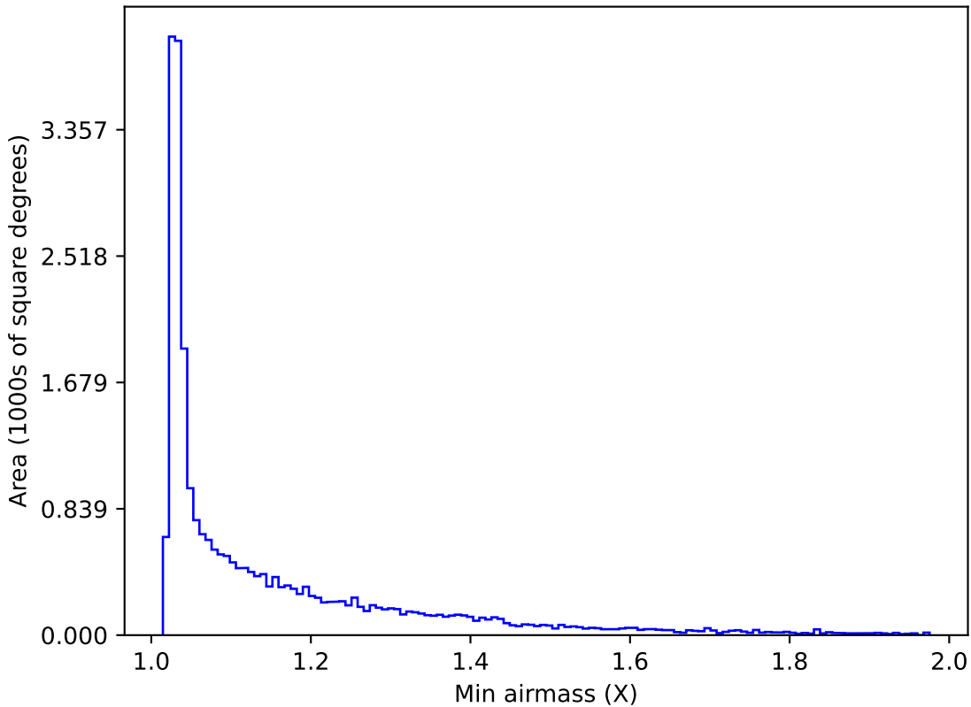
too_elab_r64_d2_griz_v3.4_10yrs Yr 1 all bands: Min airmass
