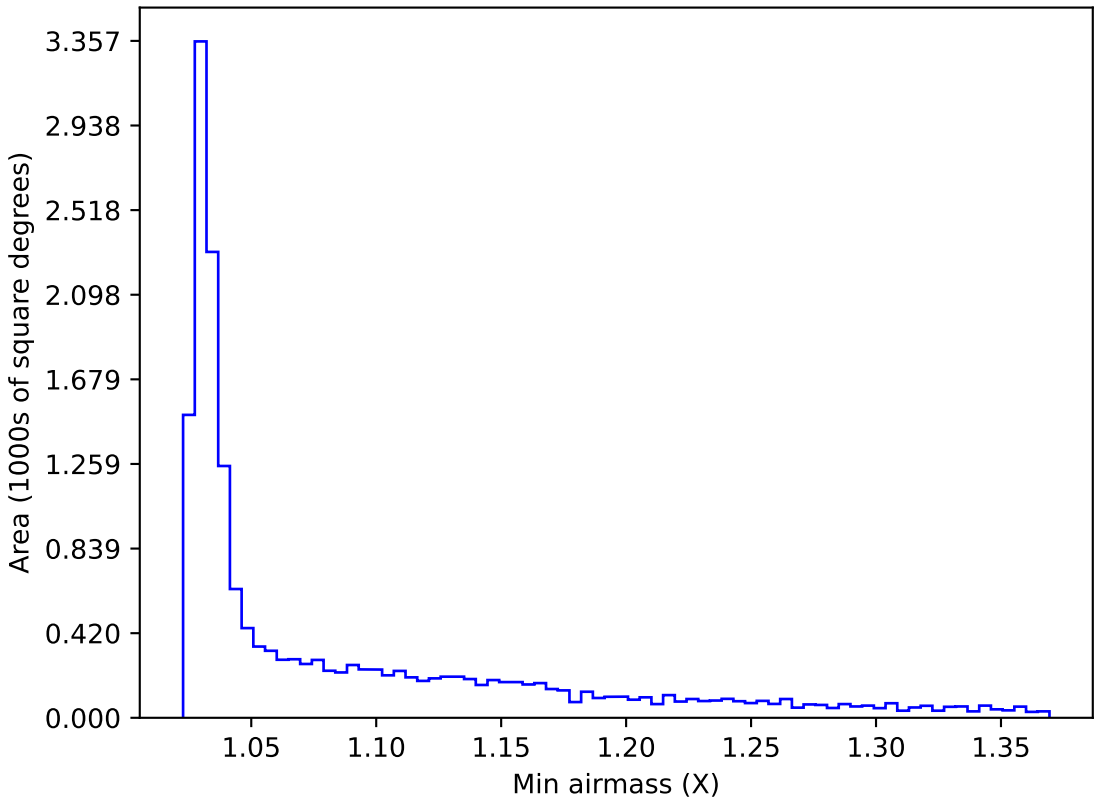
too_elab_r64_d2_griz_v3.4_10yrs WFD y band: Min airmass
