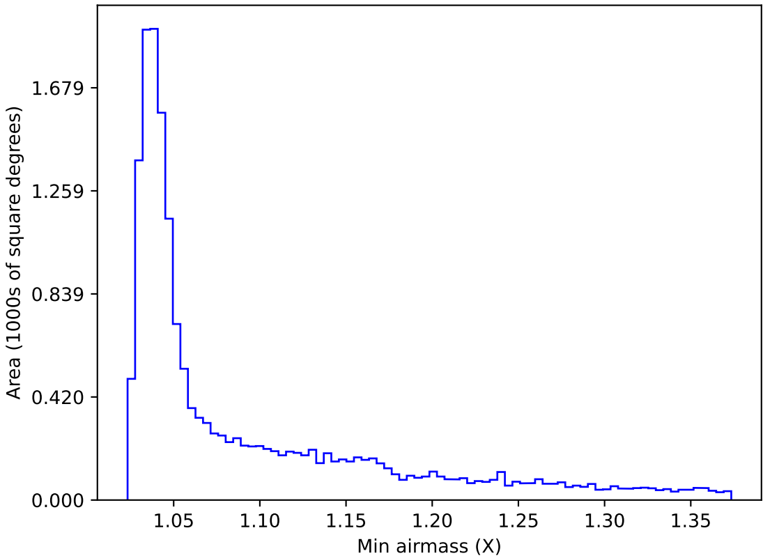
too_elab_r64_d2_griz_v3.4_10yrs WFD u band: Min airmass
