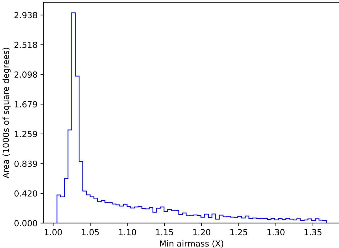
too_elab_r64_d2_griz_v3.4_10yrs WFD i band: Min airmass
