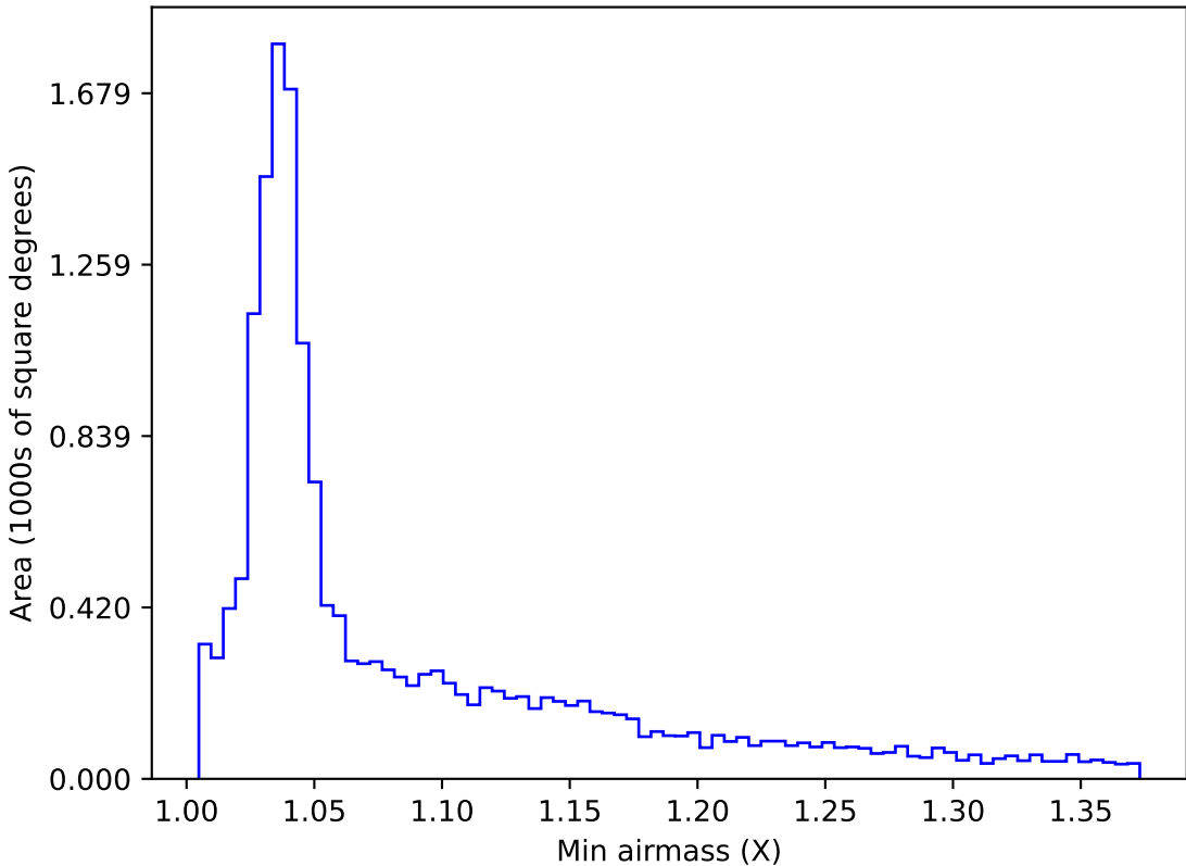
too_elab_r64_d2_griz_v3.4_10yrs WFD g band: Min airmass
