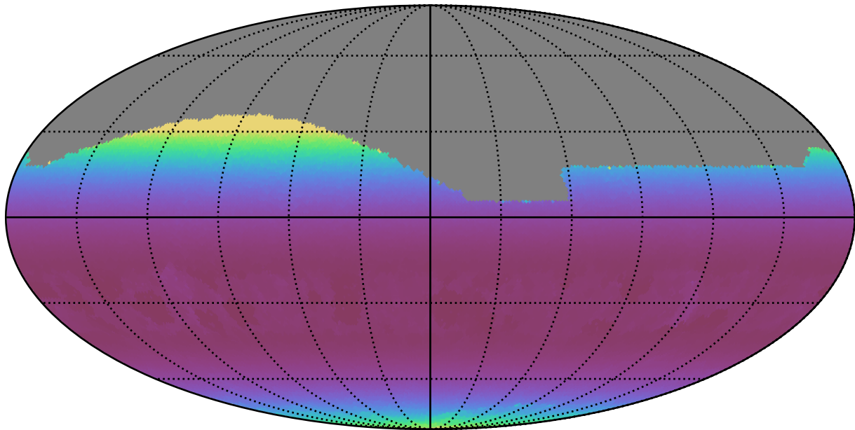
too_elab_r64_d2_griz_v3.4_10yrs All sky g band: Min airmass
