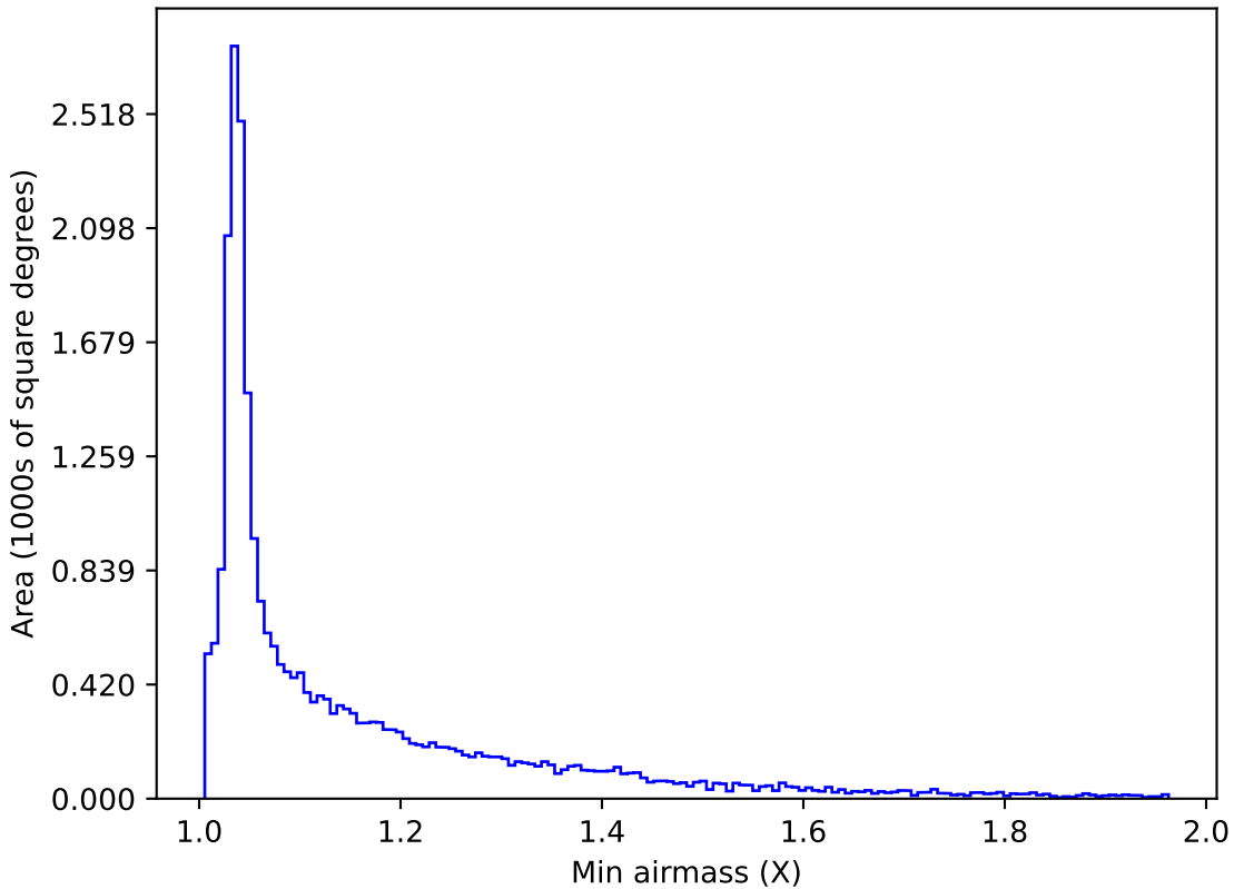
too_elab_r64_d2_griz_v3.4_10yrs All sky g band: Min airmass
