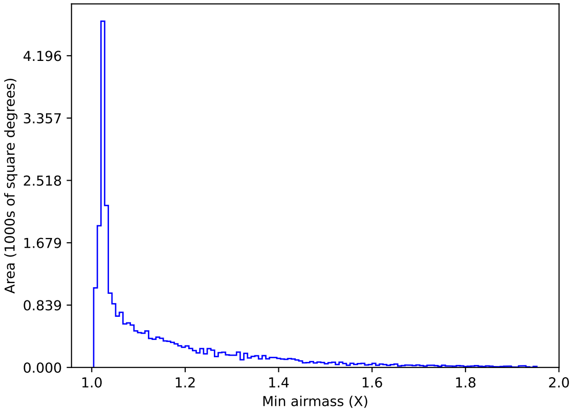
too_elab_r64_d2_griz_v3.4_10yrs All sky all bands: Min airmass
