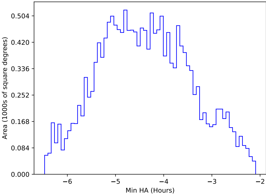
too_elab_r64_d2_griz_v3.4_10yrs WFD z band: Min HA
