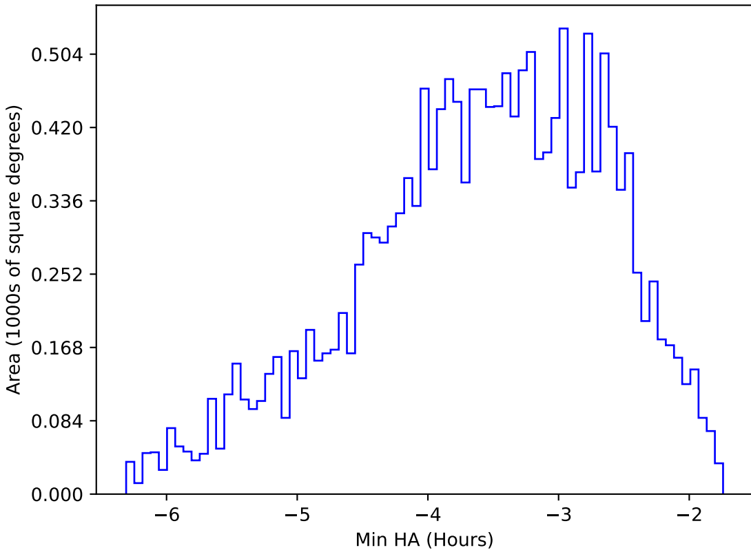
too_elab_r64_d2_griz_v3.4_10yrs WFD y band: Min HA
