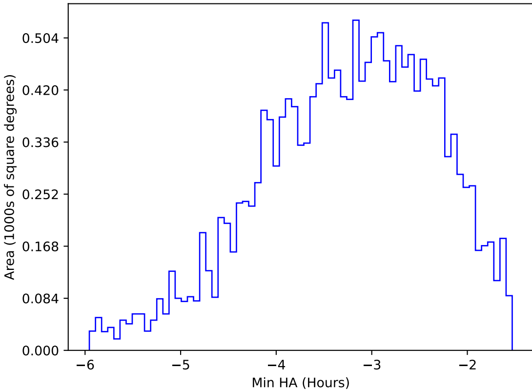
too_elab_r64_d2_griz_v3.4_10yrs WFD u band: Min HA
