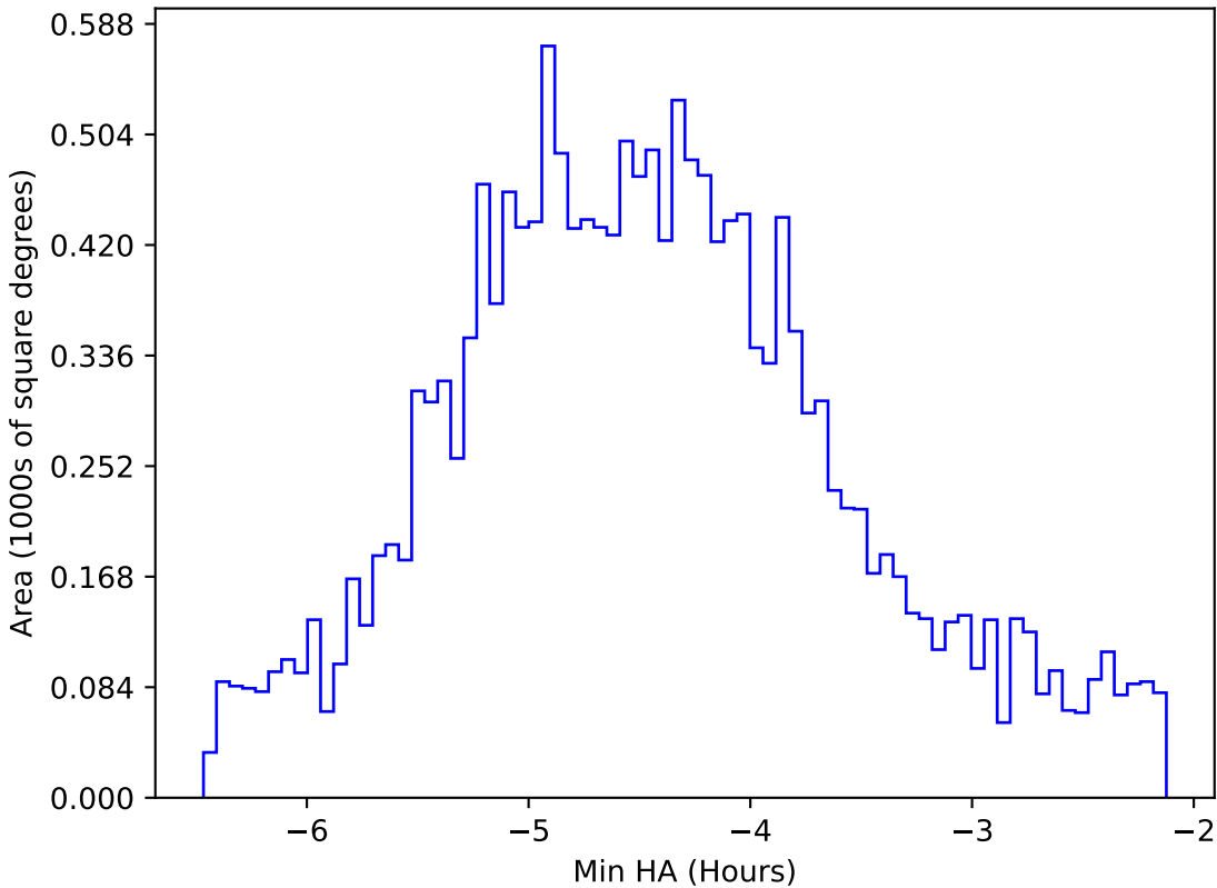
too_elab_r64_d2_griz_v3.4_10yrs WFD i band: Min HA
