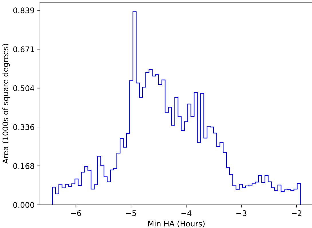
too_elab_r64_d2_griz_v3.4_10yrs WFD g band: Min HA
