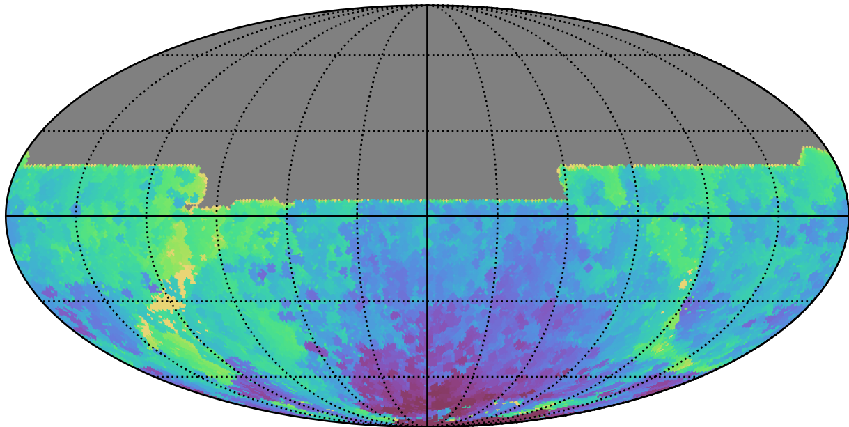
too_elab_r64_d2_griz_v3.4_10yrs All sky y band: Min HA
