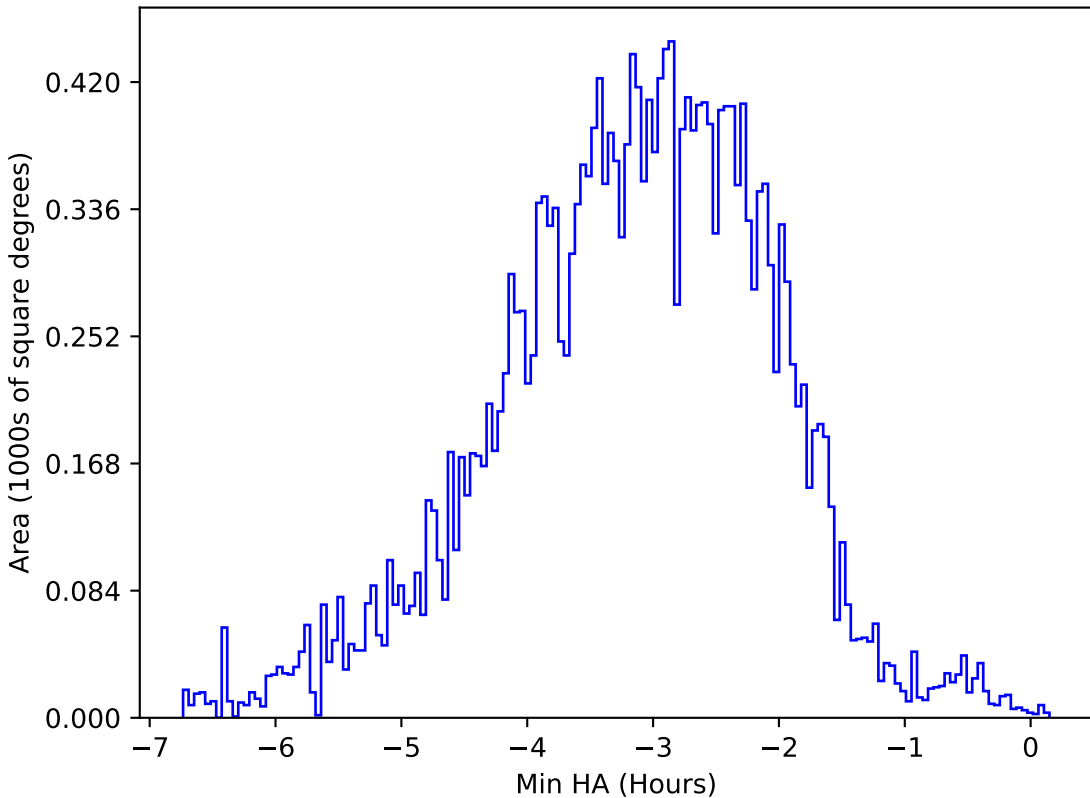
too_elab_r64_d2_griz_v3.4_10yrs All sky u band: Min HA
