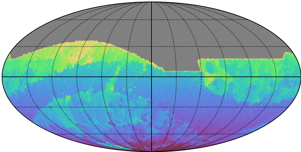
too_elab_r64_d2_griz_v3.4_10yrs All sky r band: Min HA
