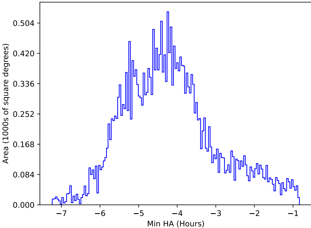
too_elab_r64_d2_griz_v3.4_10yrs All sky r band: Min HA
