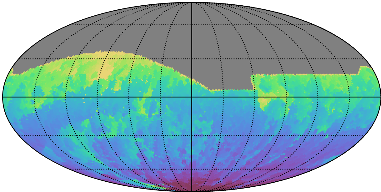
too_elab_r64_d2_griz_v3.4_10yrs All sky i band: Min HA
