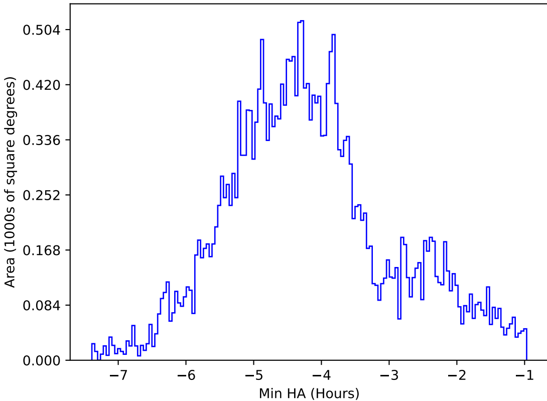
too_elab_r64_d2_griz_v3.4_10yrs All sky i band: Min HA
