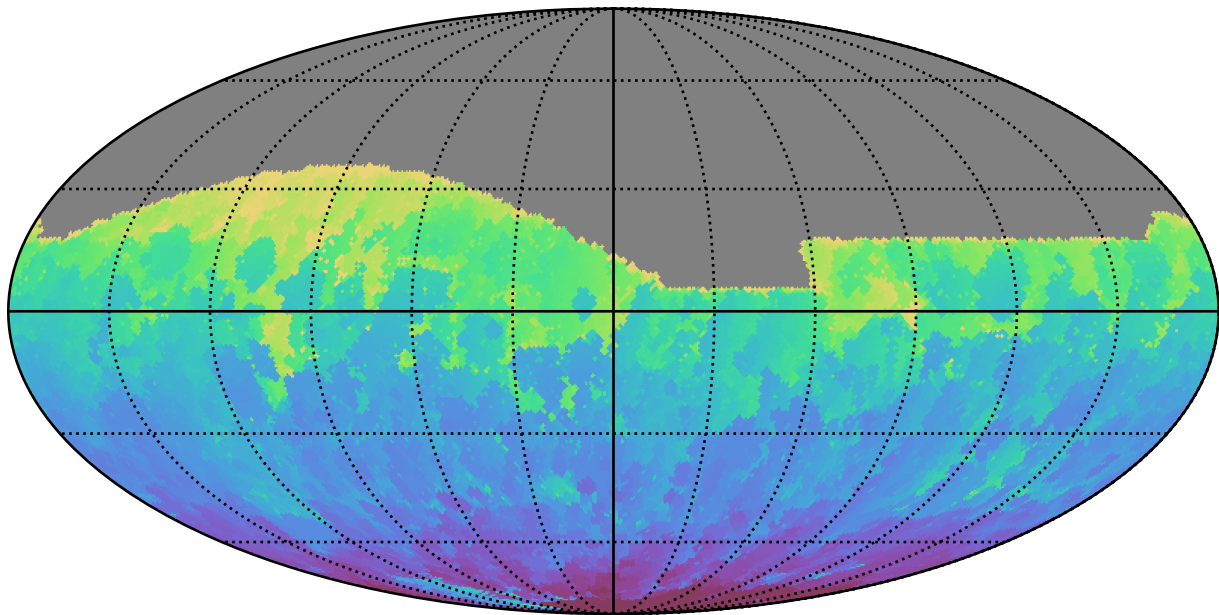
too_elab_r64_d2_griz_v3.4_10yrs All sky g band: Min HA
