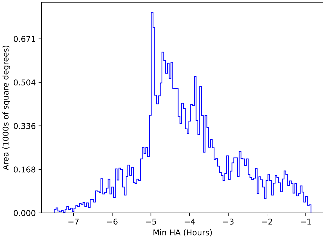
too_elab_r64_d2_griz_v3.4_10yrs All sky g band: Min HA
