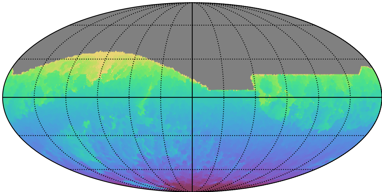
too_elab_r64_d2_griz_v3.4_10yrs All sky all bands: Min HA
