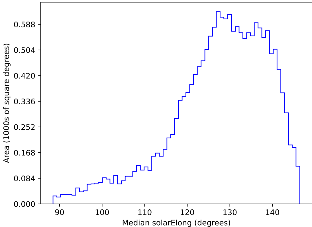
too_elab_r64_d2_griz_v3.4_10yrs WFD z band: Median solarElong
