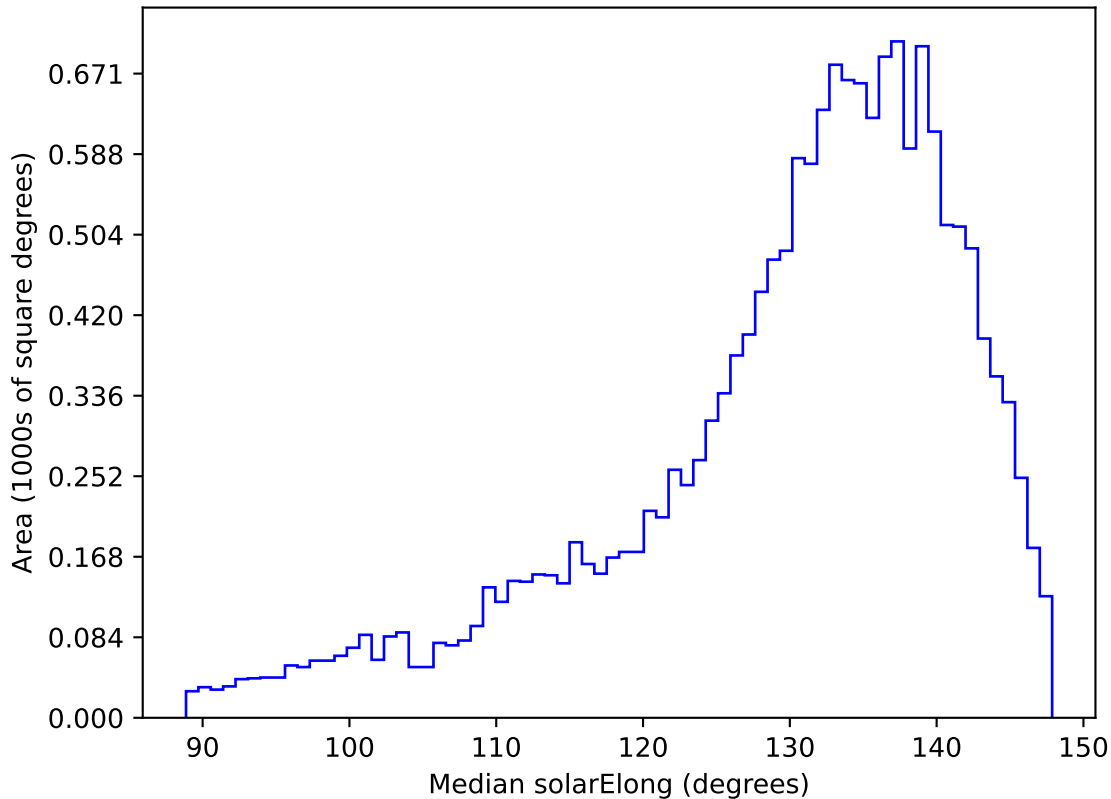
too_elab_r64_d2_griz_v3.4_10yrs WFD y band: Median solarElong
