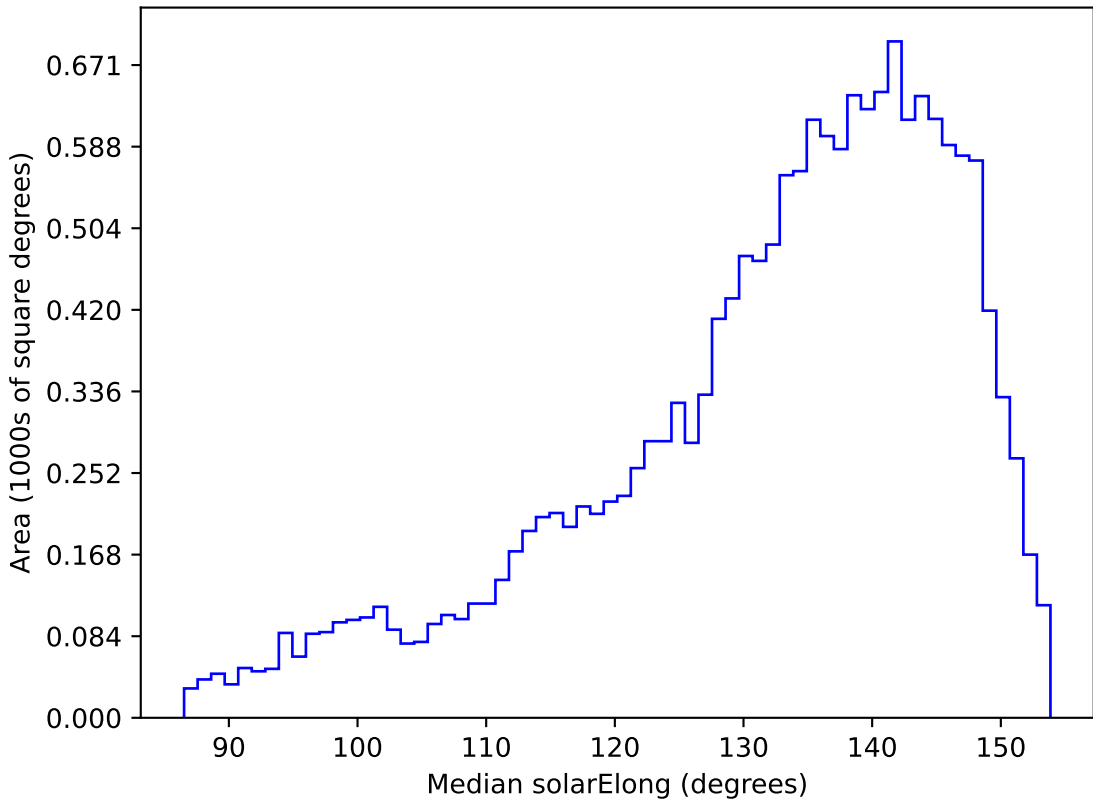
too_elab_r64_d2_griz_v3.4_10yrs WFD u band: Median solarElong
