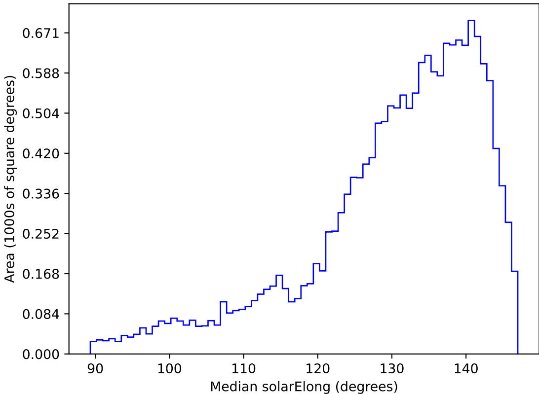
too_elab_r64_d2_griz_v3.4_10yrs WFD r band: Median solarElong
