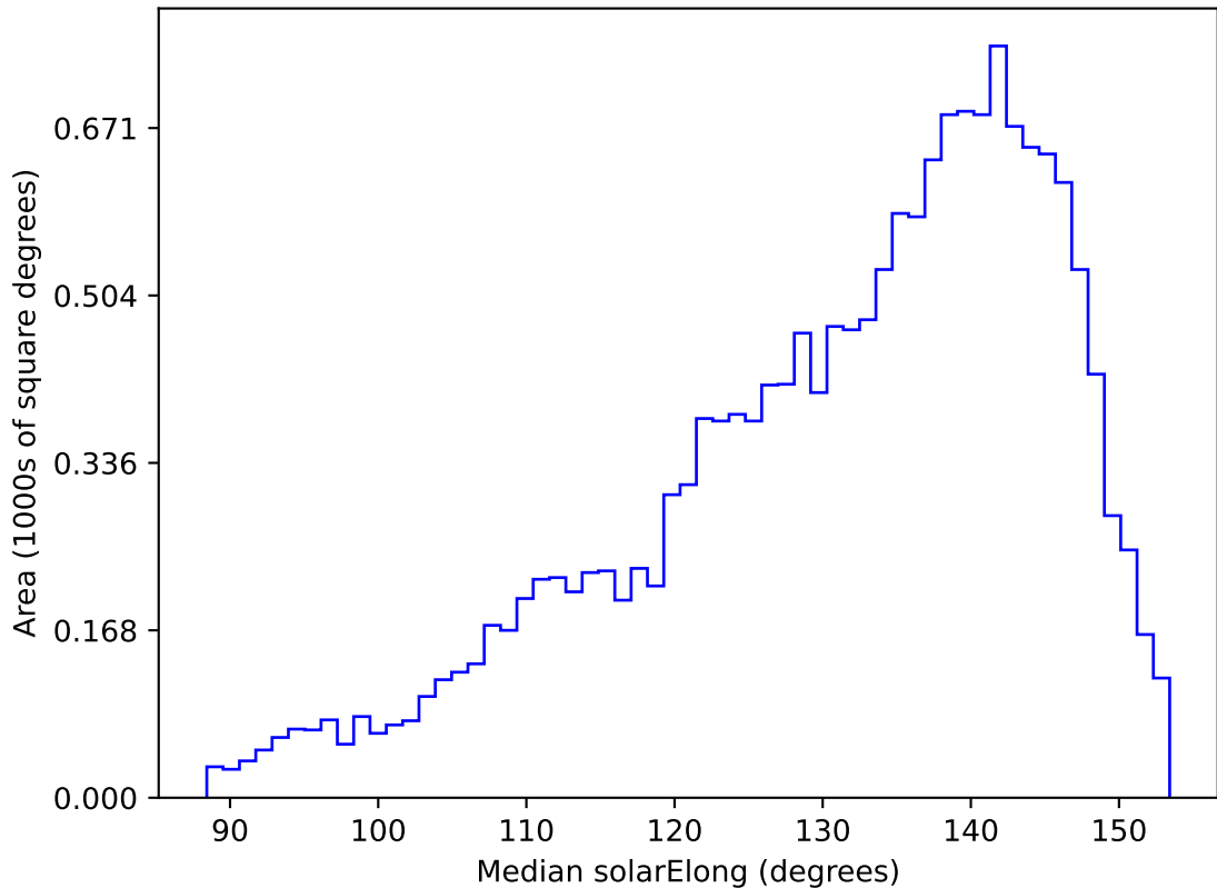
too_elab_r64_d2_griz_v3.4_10yrs WFD g band: Median solarElong
