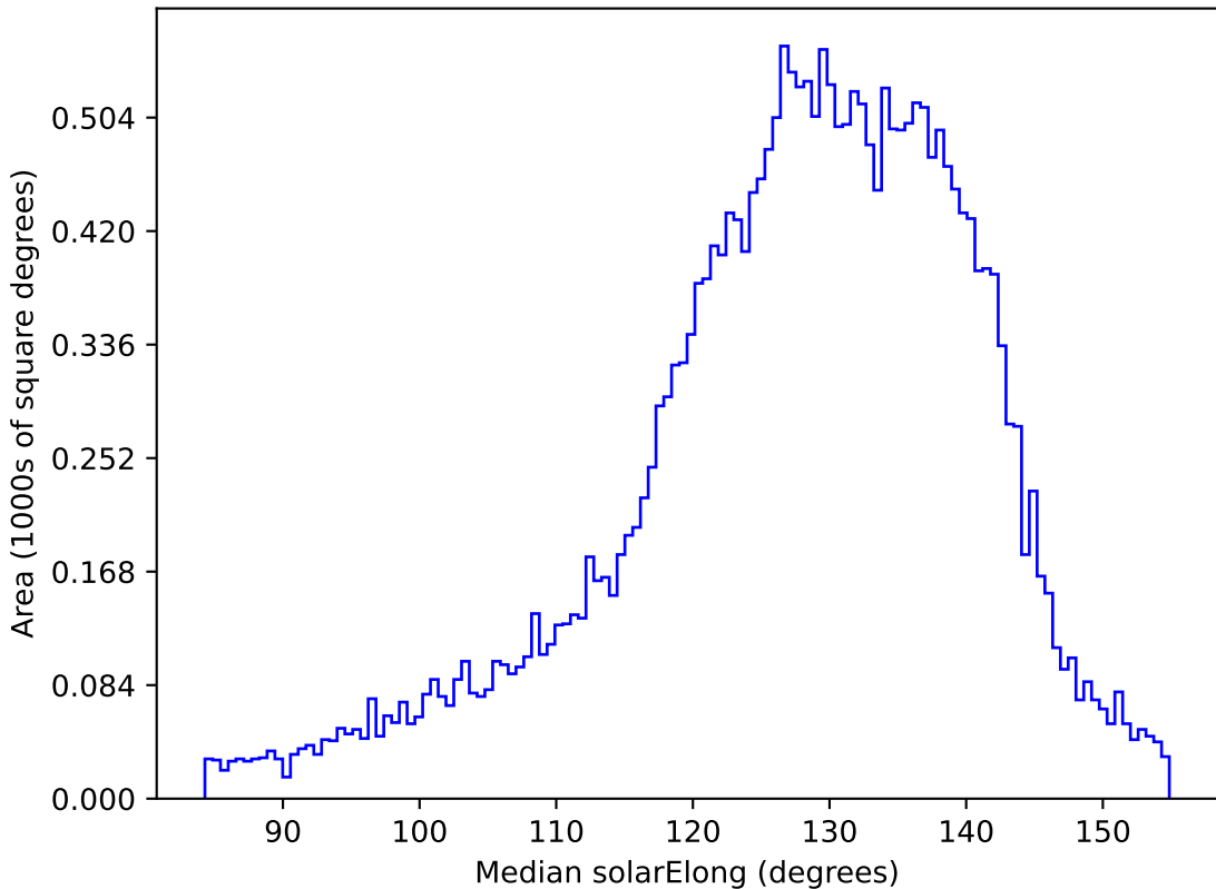
too_elab_r64_d2_griz_v3.4_10yrs All sky z band: Median solarElong
