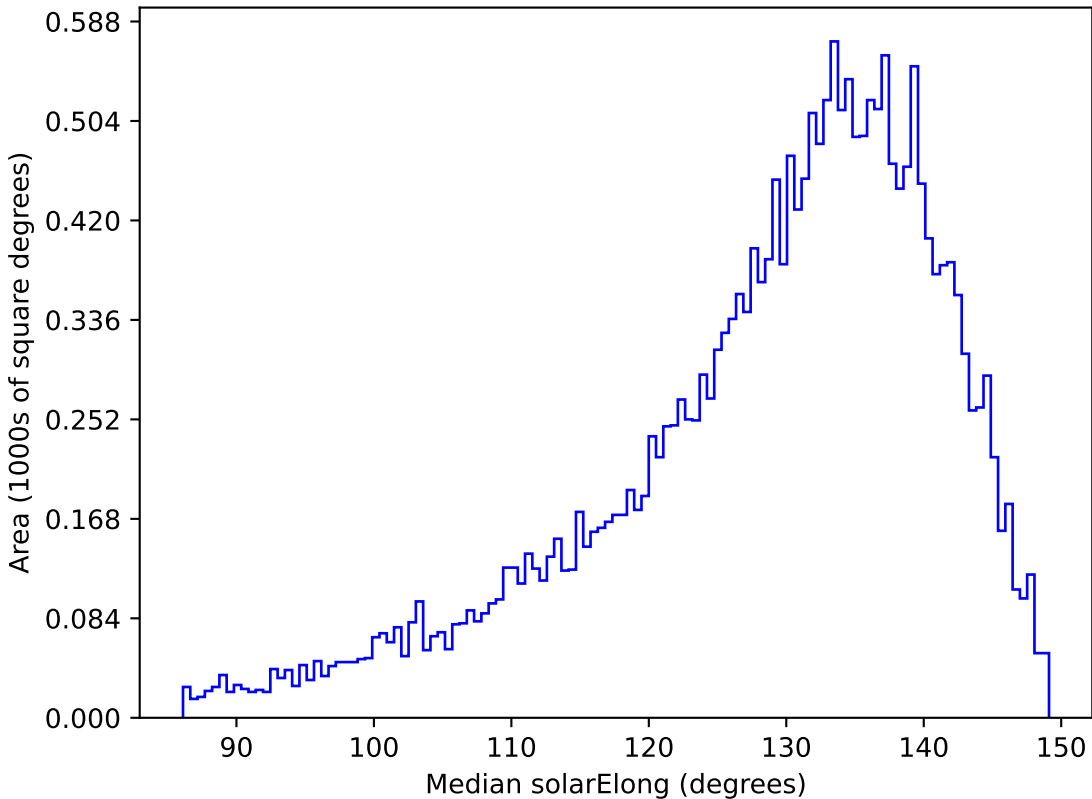
too_elab_r64_d2_griz_v3.4_10yrs All sky y band: Median solarElong
