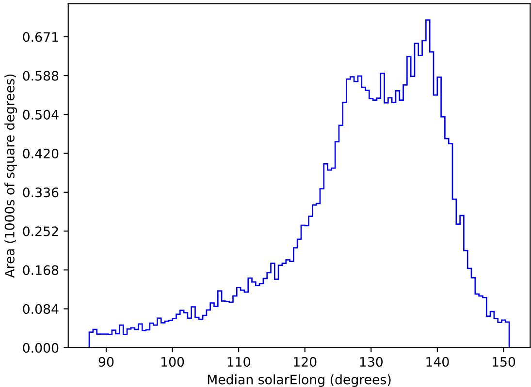
too_elab_r64_d2_griz_v3.4_10yrs All sky i band: Median solarElong
