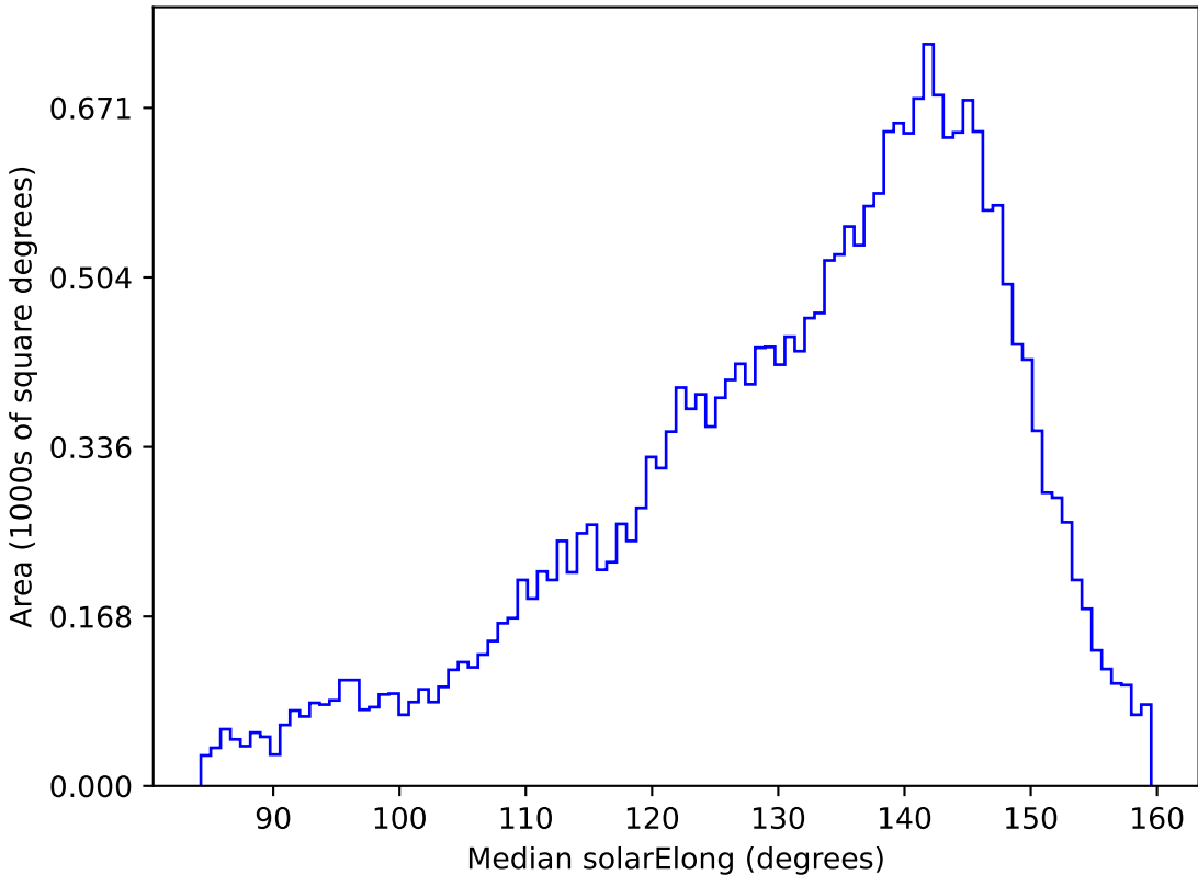
too_elab_r64_d2_griz_v3.4_10yrs All sky g band: Median solarElong
