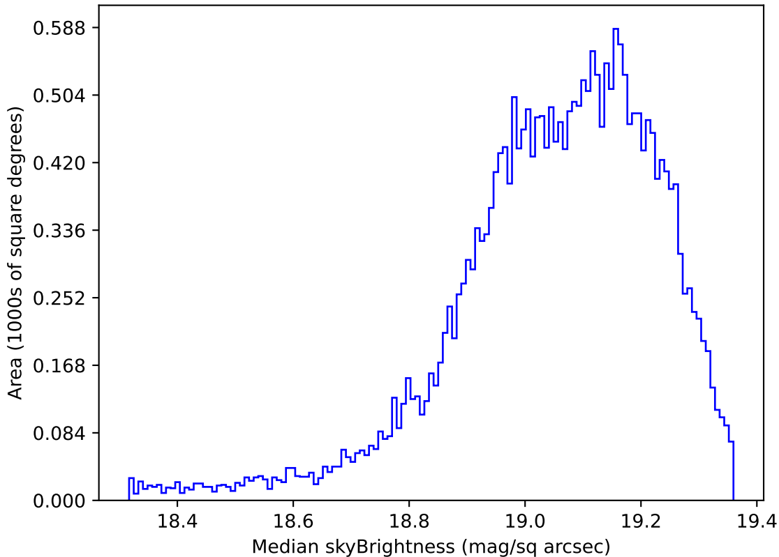
too_elab_r64_d2_griz_v3.4_10yrs Yr 1 z band: Median skyBrightness
