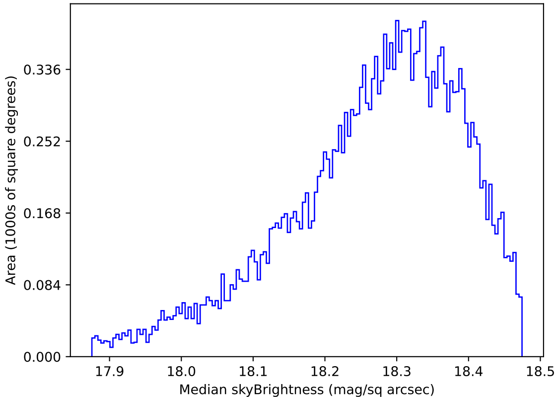
too_elab_r64_d2_griz_v3.4_10yrs Yr 1 y band: Median skyBrightness
