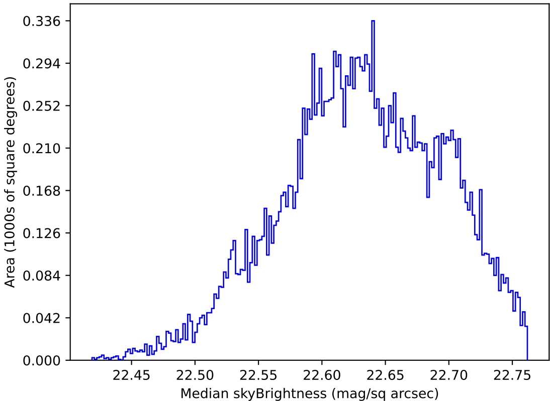
too_elab_r64_d2_griz_v3.4_10yrs Yr 1 u band: Median skyBrightness
